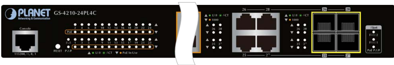
Figure 2-1-2b GS-4210-24P (L) 4C LED Panel
